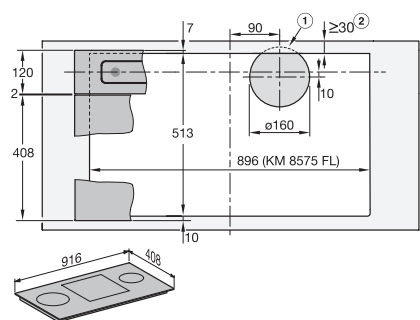
DAD4370, DAD4870, DAD4970, DAD6880, DAD6980, Installation drawings
