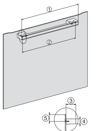
H7000 handle, glass, installation drawings
