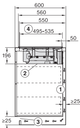
KMDA7272-1FL, KMDA7473-1FL/FL MattFinish, KMDA7272FL, KMDA7473FL – Side view lying on top, Plug&Play
