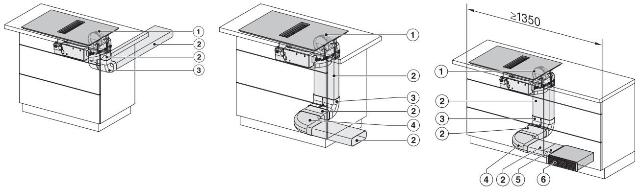
KMDA7676-1FL, KMDA7876-1FL, KMDA7676FL, KMDA7876FL – Installation variant 2 Basis
